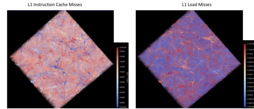
In-Situ instrumenting of HACC with performance Data
